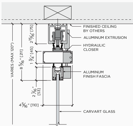
HYDRAULIC DOOR HEADER @ MID-RUN PANEL DOOR
